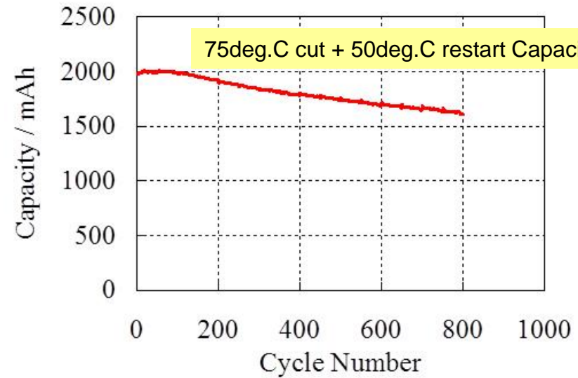
20A discharge cycle
